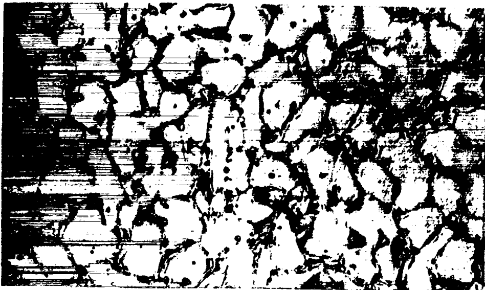
Figure 3. Example 2. Plutonium-1 w/o gallium delta alloy, rolled and then recrystallized. Similar to Figure 2 except for the finer grain size. 500 X.
